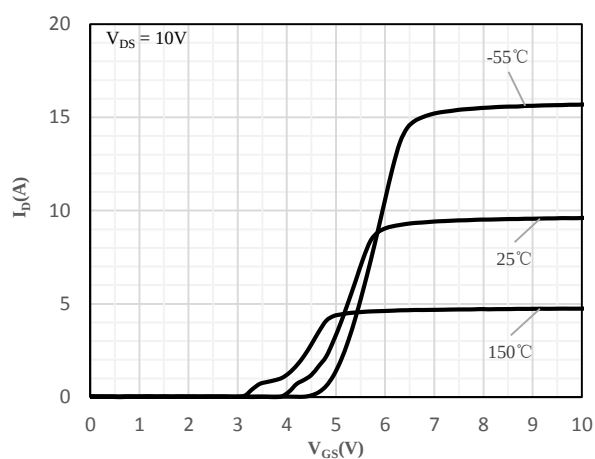
Fig 8 Transfer Characteristics
